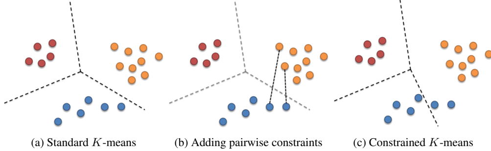
Figure 2: Illustration of our constrained clustering framework. (a) Standard K -means has only one feature type; (b) we add more feature types, which induce pairwise soft constraints between instances; (c) CRF inference balances evidence from all features in performing the clustering.
